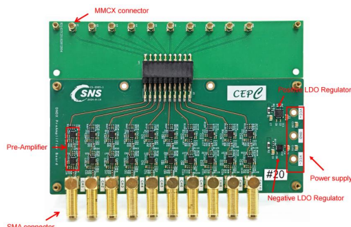
10-channel pre-amplifier board (left) and the 40-channel crate in the lab (right)
