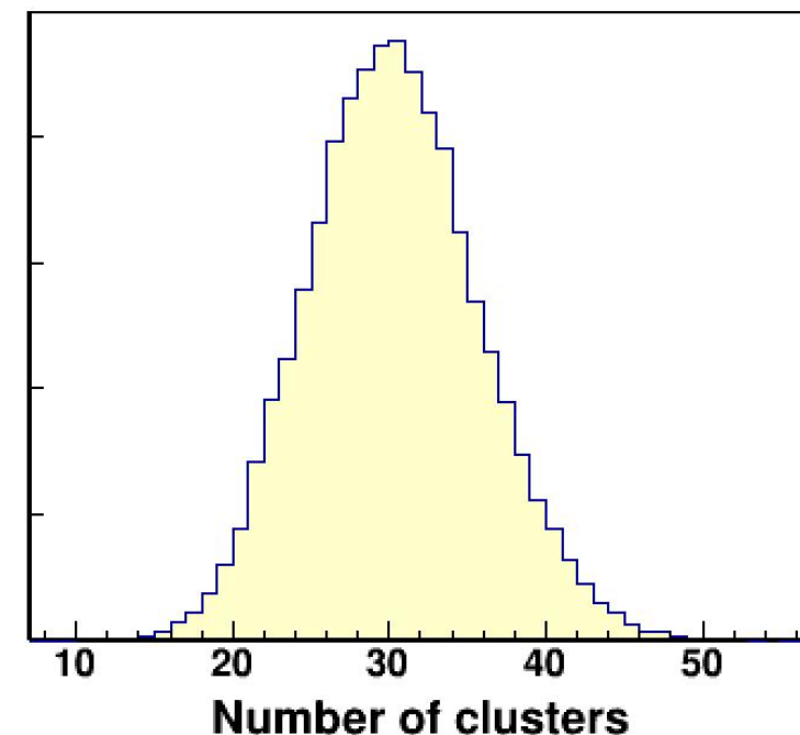
dN/dx : clusters per unit length
