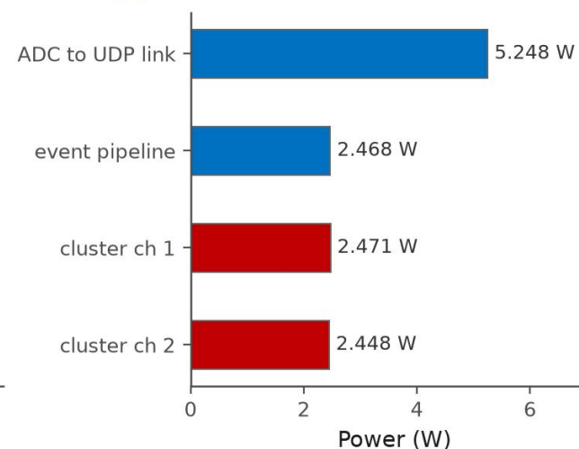
(c) On-chip power, total 12.37 W
