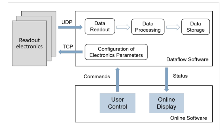
DAQ system
