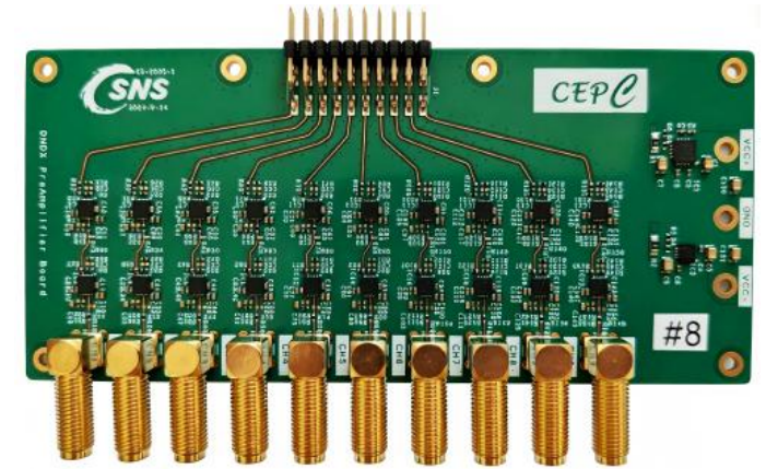
Preamplifier
