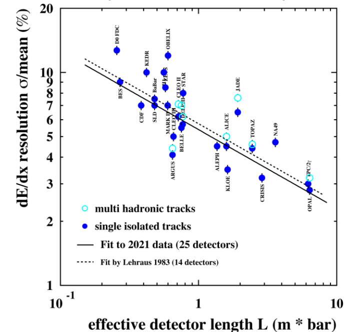
Lehraus plot (from Michael Hauschild)
