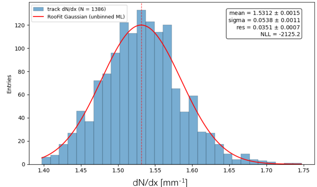
dN/dx (L=1.2m track)
