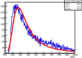
Layer7_Chip2_Chn10
