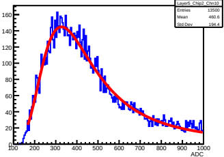
Layer5_Chip2_Chn10
