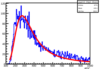
Layer13_Chip2_Chnl13
