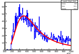
Layer9_Chip2_Chnl7
