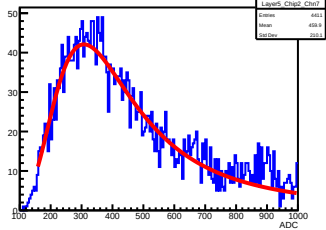
Layer5_Chip2_Chn7
