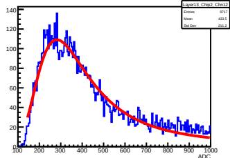
Layer13_Chip2_Chnl12
