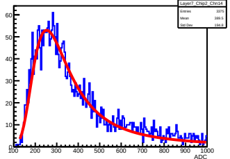
Layer7_Chip2_Chnl4
