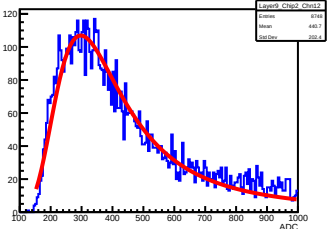
Layer9_Chip2_Chnl12
