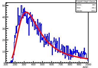
Layer9_Chip2_Chnl14
