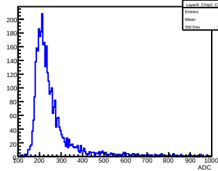
Layer 8, Chip 2, Channel 23
