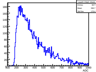
Layer 9, Chip 3, Channel 21
