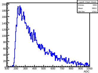
Layer 6, Chip 3, Channel 22
