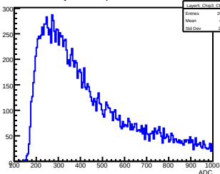
Layer 5, Chip 3, Channel 19
