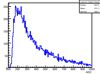
Layer 13, Chip 3, Channel 18
