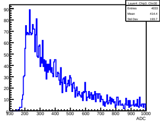
Layer 4, Chip 3, Channel 30
