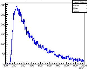
Layer 5, Chip 3, Channel 23
