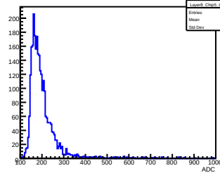
Layer 8, Chip 5, Channel 15
