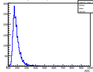
Layer 19, Chip 1, Channel 11
