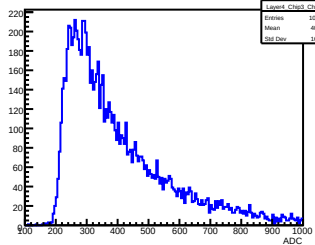
Layer 4, Chip 3, Channel 19
