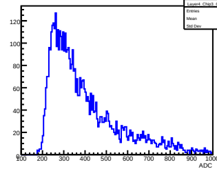
Layer 4, Chip 3, Channel 14
