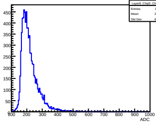
Layer 8, Chip 5, Channel 18
