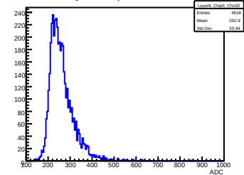
Layer 8, Chip 0, Channel 20
