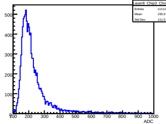
Layer 8, Chip 3, Channel 8
