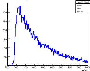
Layer 23, Chip 3, Channel 23
