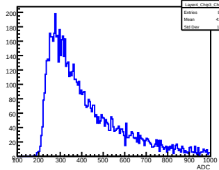
Layer 4, Chip 3, Channel 20
