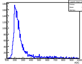
Layer 8, Chip 2, Channel 24
