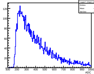
Layer 7, Chip 3, Channel 26
