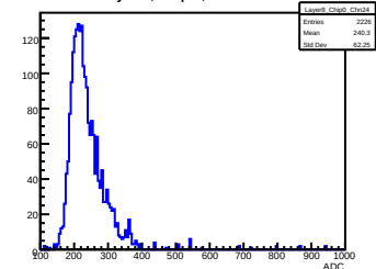
Layer 8, Chip 0, Channel 24
