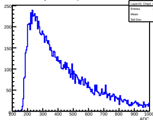
Layer 23, Chip 3, Channel 15
