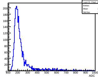
Layer 19, Chip 2, Channel 20
