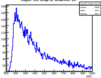
Layer 19, Chip 3, Channel 12
