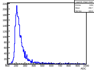
Layer 19, Chip 4, Channel 8
