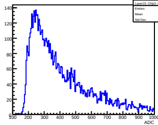
Layer 23, Chip 3, Channel 11
