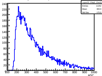
Layer 23, Chip 3, Channel 22
