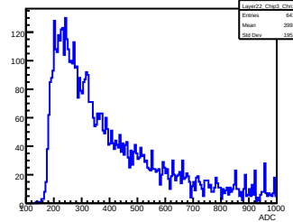
Layer 22, Chip 3, Channel 31
