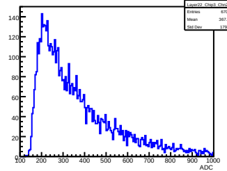
Layer 22, Chip 3, Channel 28
