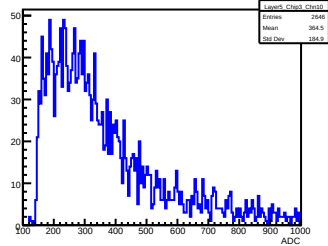
Layer 5, Chip 3, Channel 10
