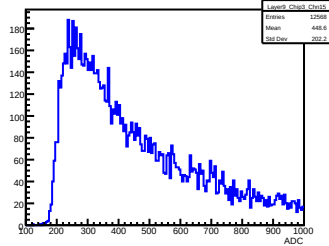
Layer 9, Chip 3, Channel 15
