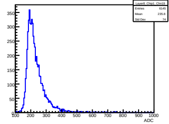
Layer 8, Chip 1, Channel 19
