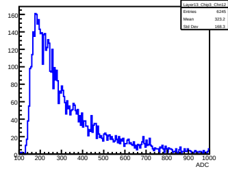
Layer 13, Chip 3, Channel 12
