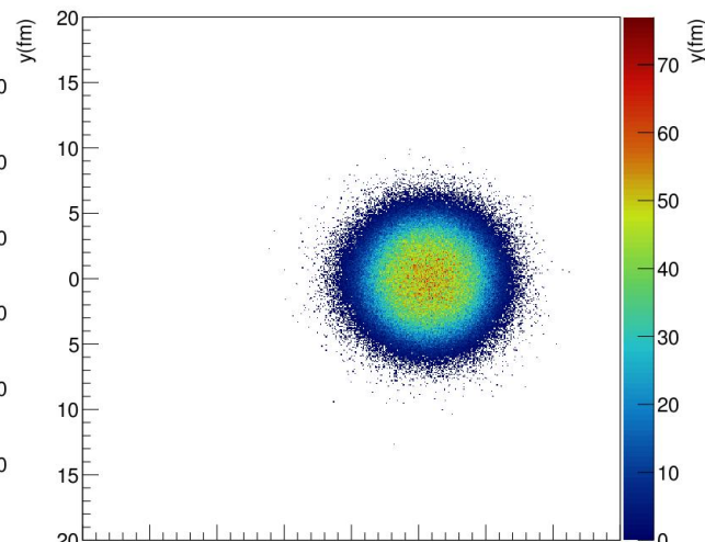
RuRu_proton_project
