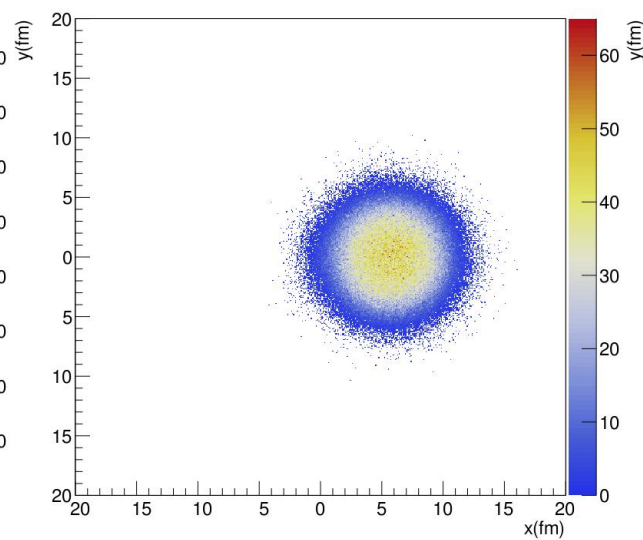
RuRu_proton_project
