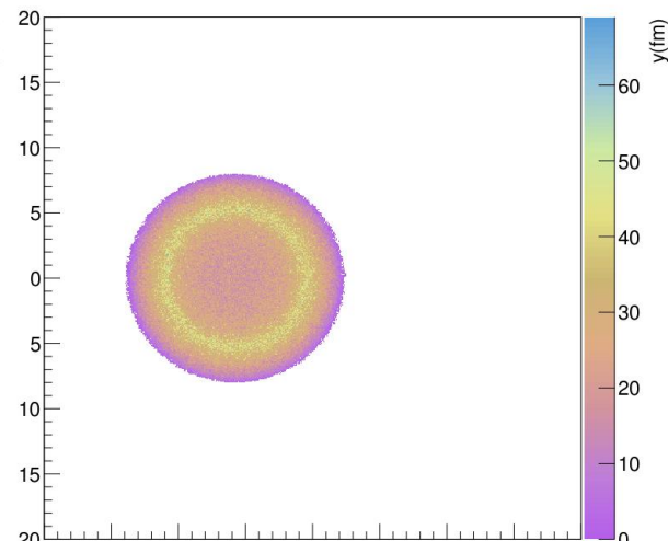
ZrZr_proton_target
