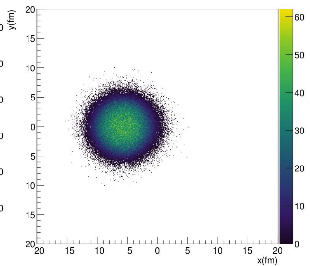
RuRu_proton_target
