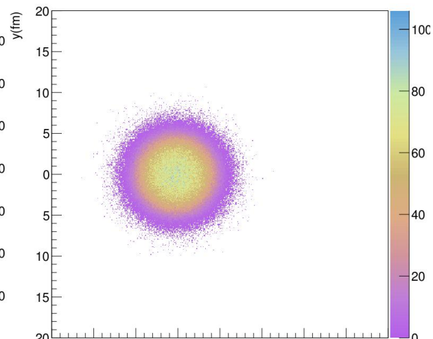
RuRu_proton_target
