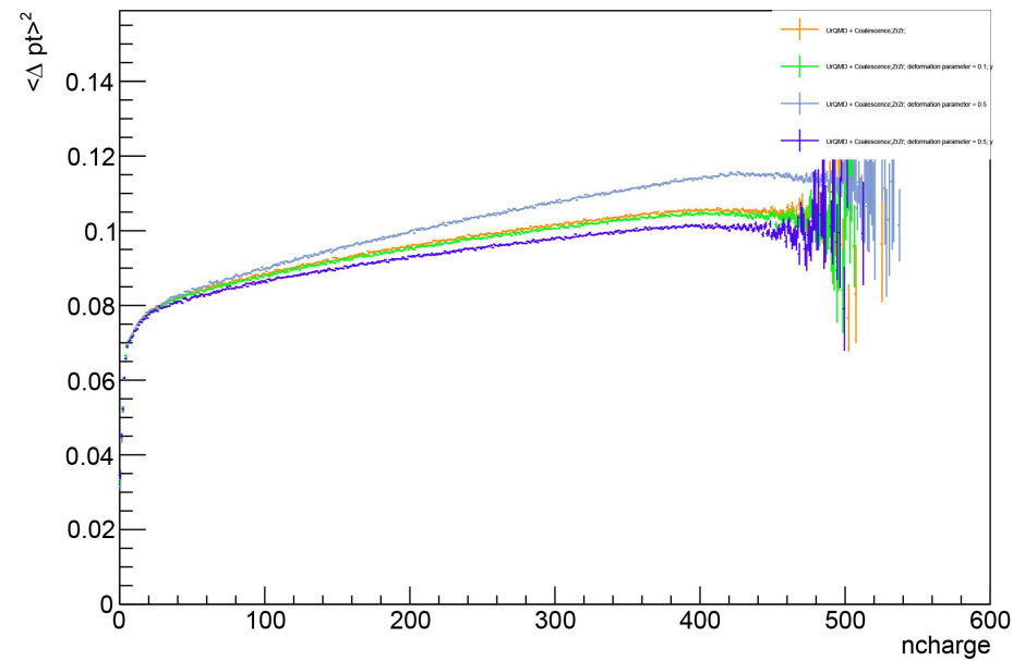
\langle \Delta p_t^2 \rangle vs ncharge
