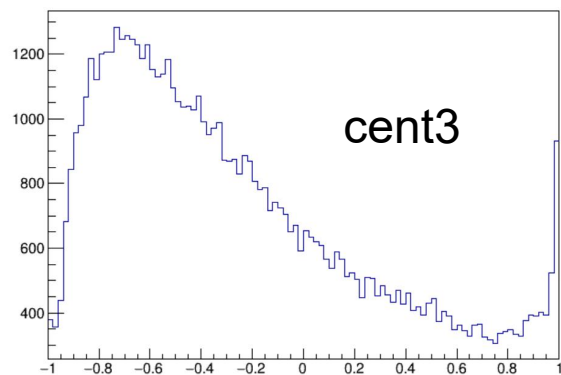
LambdaCosThetaHX_vs_cent
