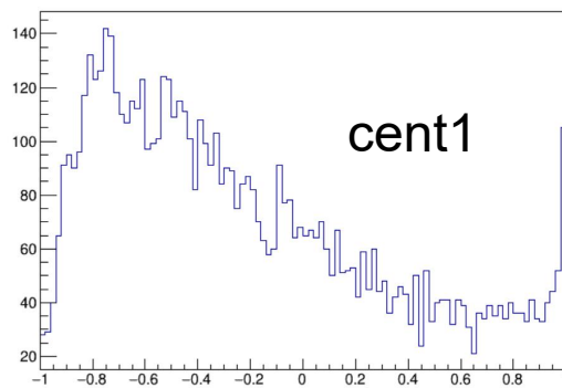
LambdaCosThetaHX_vs_cent
