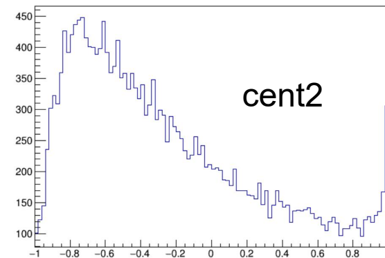
LambdaCosThetaHX_vs_cent
