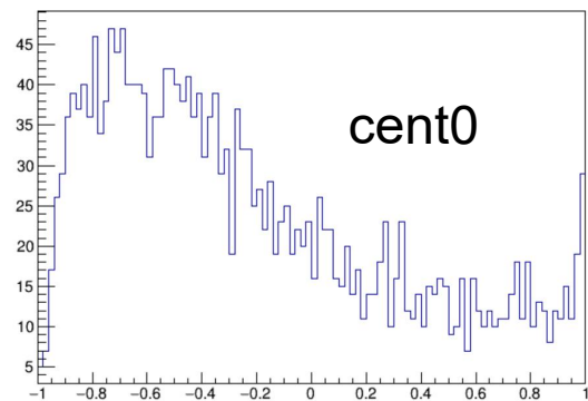
LambdaCosThetaHX_vs_cent
