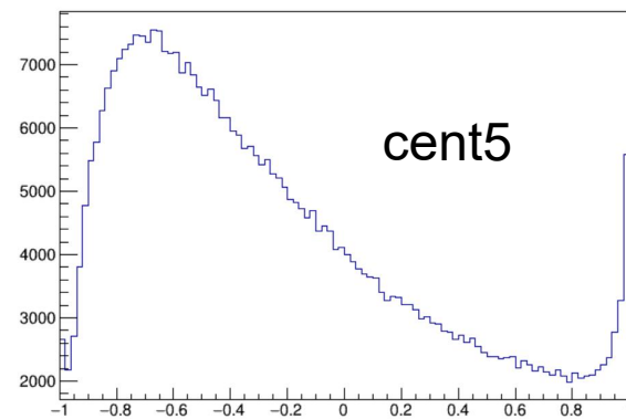
LambdaCosThetaHX_vs_cent
