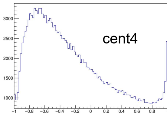
LambdaCosThetaHX_vs_cent
