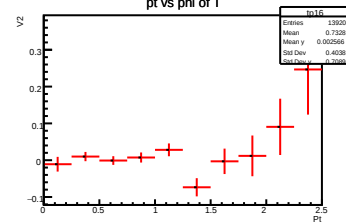
pt vs phi of T
