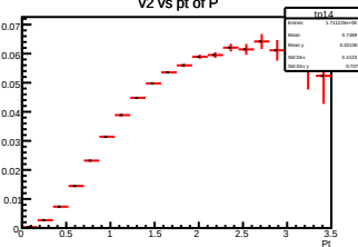
v2 vs pt of P
