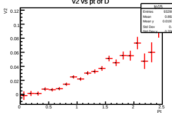
v2 vs pt of D
