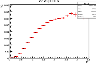
v2 vs pt of N
