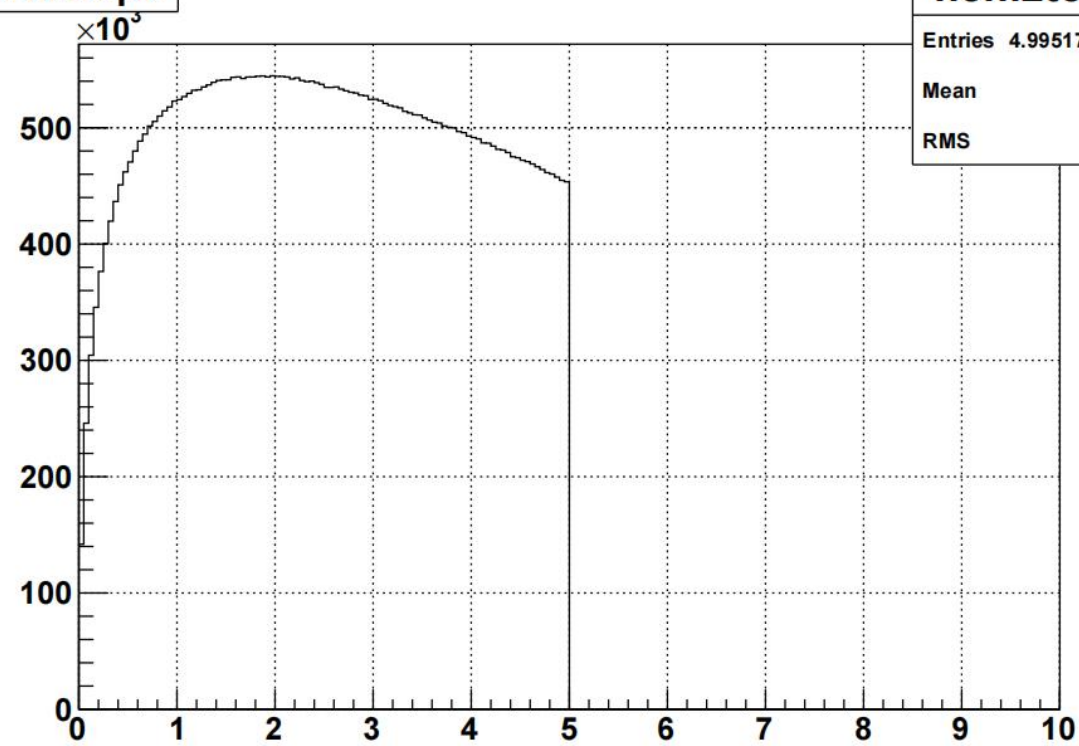
hchi2topo
