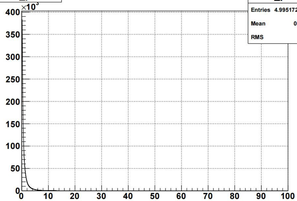
hdca_proton
