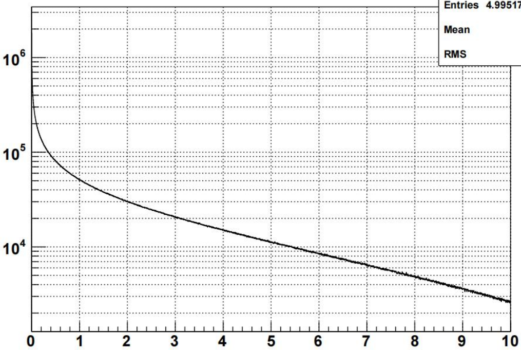
hchi2ndf
